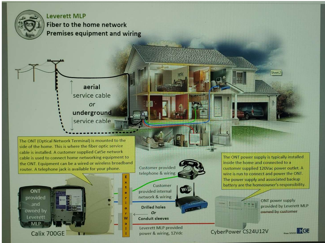
Fiber-to-the-home premises equipment and wiring.
